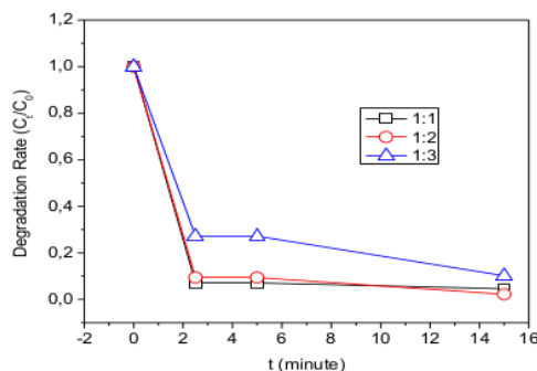
Figure 11. Degradation Rate ( C_t/C_0 ) of \text{Fe}_3\text{O}_4/\text{rGO} Samples
