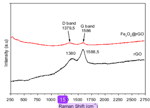
Figure 5. Raman shift of rGO and \text{Fe}_3\text{O}_4/\text{rGO}
