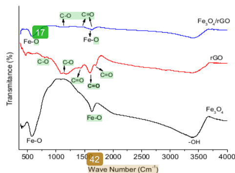
Figure 3. FTIR of: \text{Fe}_3\text{O}_4 , rGO, and \text{Fe}_3\text{O}_4/\text{rGO}
