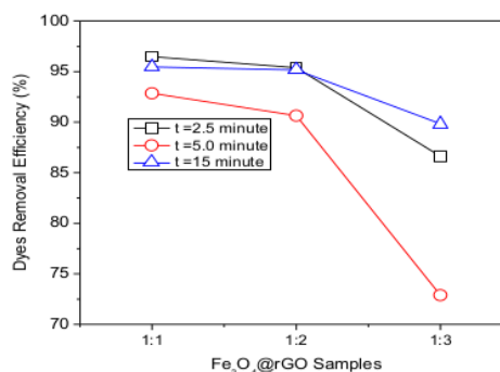
Figure 10. Dyes Removal Efficiency ( \text{DRE}_{\text{MB}} ) by \text{Fe}_3\text{O}_4/\text{rGO} Core-shell
