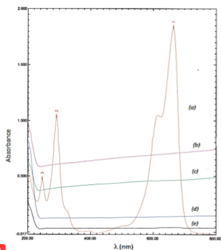
Figure 8. UV-Vis Spectra of: (a) MB and (b-e) MB/ \text{Fe}_3\text{O}_4/\text{rGO} (#1:4, #1:3, #1:2 and #1:1) after 2.5 min
